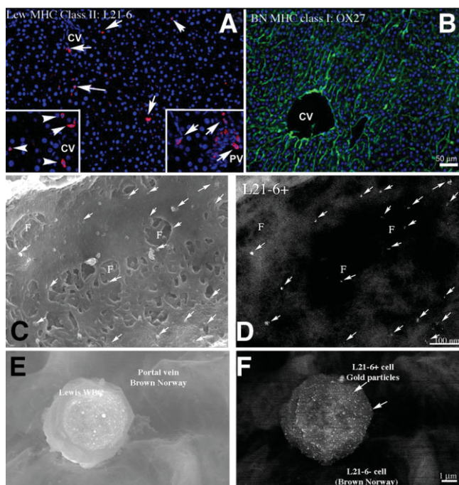
Fig. 5. Evaluation of recipient LEW cells in BN liver. (A) LEW-specific MHC class II antibody (L21-6) identified LEW cells in the BN donor liver 3 days post-OLTx. Few cells are observed in the sinusoids of the liver (red, arrows), and these cells do not show the flattened shape typical of LSECs. Higher concentrations of L21-6 + cells are found in perivascular areas surrounding the central vein (CV, left insert, arrowheads) and in the portal triad (PV, right insert, arrows) but are not integrated into the large vessel intima. (B) Control. BN MHC class I staining of most cell membranes in the transplanted BN rat liver is shown (green). High-resolution immuno-SEM evaluation of an engrafted LSEC of recipient origin was then undertaken. (C) Secondary electron image and (D) parallel backscattered electron image identify the recipient-specific surface marker L21-6 (arrows, 15-nm gold particles) on the surface of a fenestrated LSEC in the BN donor liver sinusoid. Gold particles are on the LSEC, not under the fenestrations. This positive result was seen in 1 out of several hundred cells examined using this technique, indicating it is an uncommon event. (E, F) Secondary electron image and parallel backscattered electron image, respectively, of the typical shape of an L21-6 positive cell in the liver vasculature. This cell is most likely a leukocyte.
