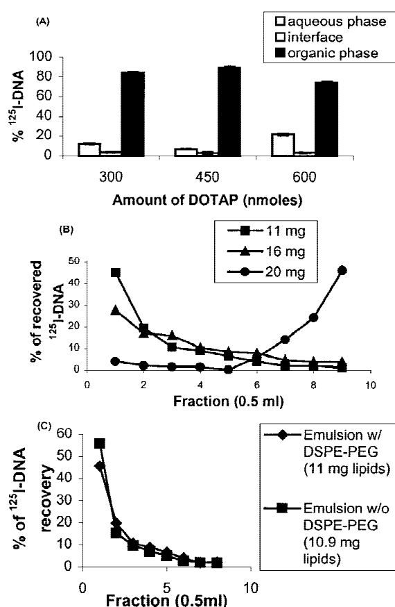
Fig. 1. (A) Effect of DOTAP on the partition of DNA into organic phase. ^{125}\text{I} -DNA (100 \mu\text{g} ) was incubated with indicated amounts of DOTAP in the Bligh and Dyer monophasic system at room temperature for 30 min. The monophasic system was separated into two phases by the addition of \text{CHCl}_3 and water. Partition of DNA into the aqueous phase, the interface and the organic phase were determined by measuring the radioactivity. (B) Sucrose density gradient sedimentation profile of DNA incorporated into emulsion containing PE-PEG with increasing amount of total emulsion lipid. (C) Sucrose density gradient sedimentation profiles of DNA incorporated into emulsion with and without PE-PEG.
